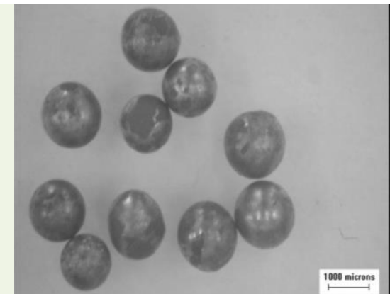
Beryllium Pebbles prepared by Rotating Electrode process
