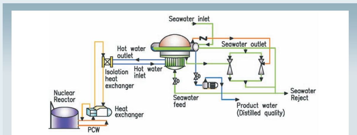
LTE Desalination using waste Heat
