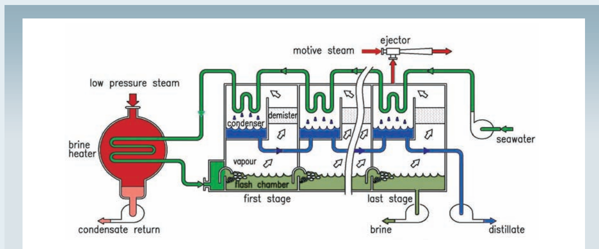
Schematic Diagram of Multi-Stage Flash (MSF) Process
