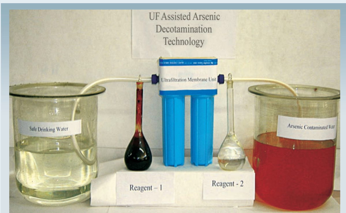
UF Assisted Arsenic Removal System
