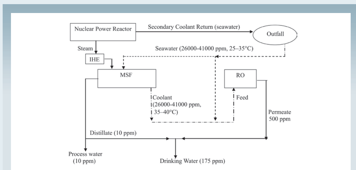
Hybrid Desalination System Integrated with Nuclear Power Reactor
