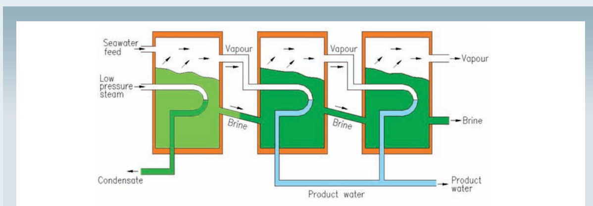
Schematic Diagram of Multi-Effect Distillation (MED) Process
